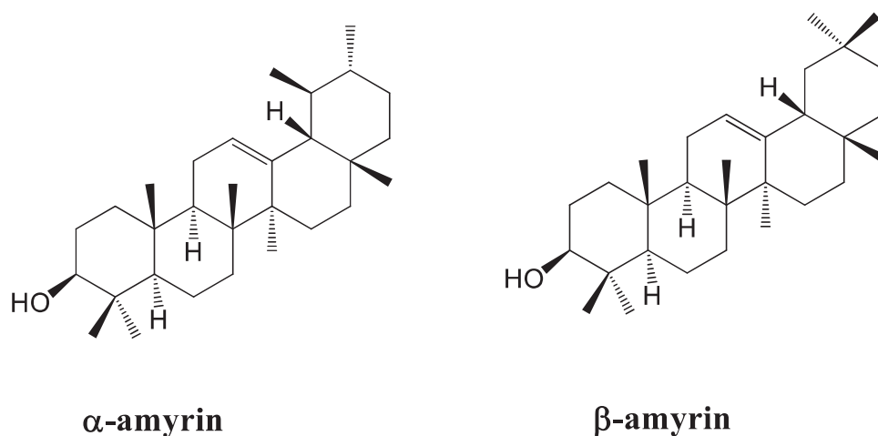
Fig. 9. Structure of \alpha -amyrin and \beta -amyrin .
