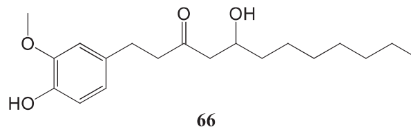
8-Gingerol
