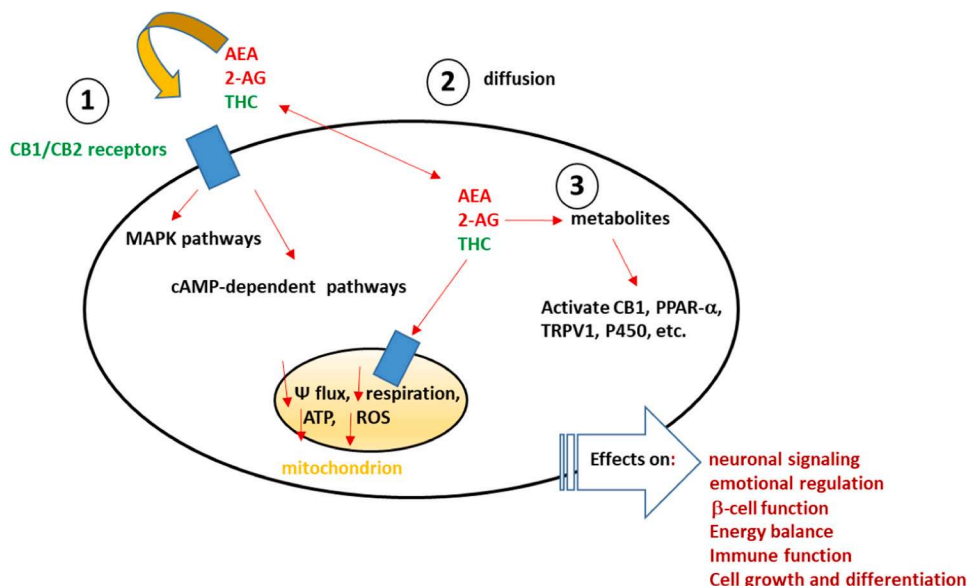
Fig. 2. Possible mechanisms of cannabinoid-like active compounds.
