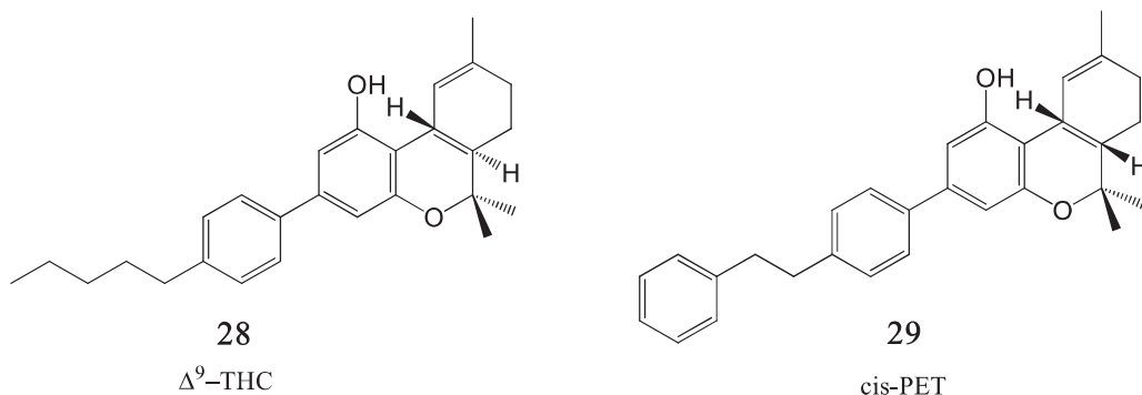
Fig. 6. Structural analogies between \Delta^9 -THC and cis-PET.
