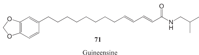
Fig. 15. Structure of Guineensine.
