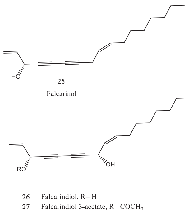
Fig. 5. Falcarinol and Falcarindiol derivatives chemical structures.
