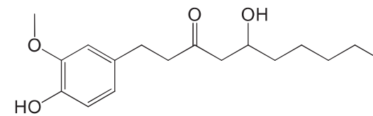
6-Gingerol
