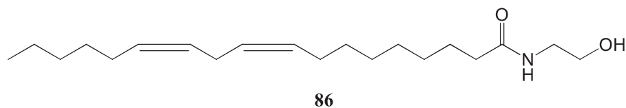
N-linoleylethanolamine
