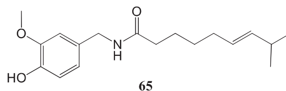
Capsaicin
