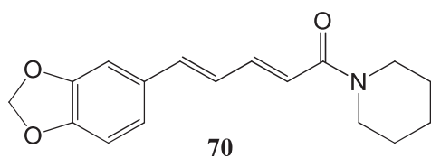
Piperine
