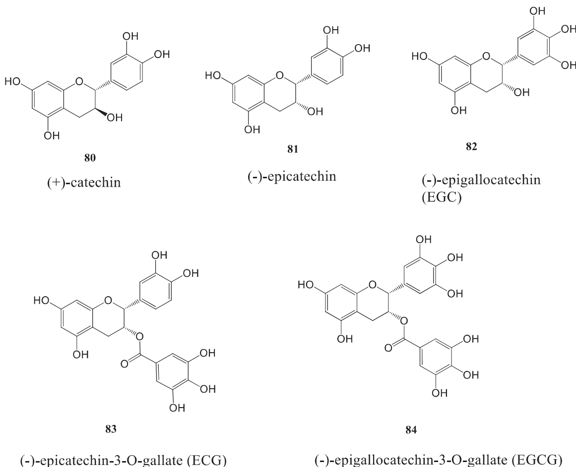
Fig. 18. Most abundant compounds found in Camellia Sinensis .
