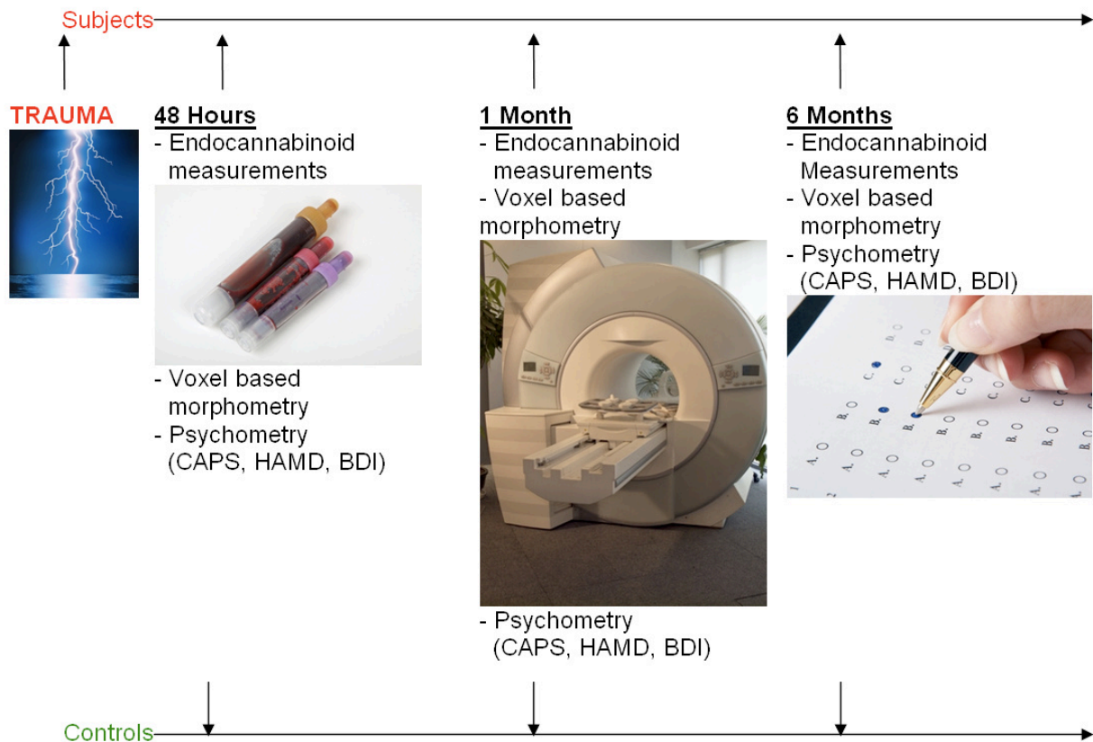
Figure 4: Study design
