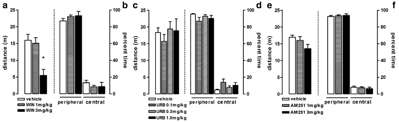
Fig. 2. (a) Effect of ip injection of WIN55,212-2 (0, 1 or 3 mg/kg) on total distance traveled and (b) percent time spent in peripheral and central zones in the open-field (n = 5/group). (c) Effect of ip injection of URB597 (0, 0.1, 0.3, or 1 mg/kg) on total distance traveled and (d) percent time spent in peripheral and central zones in the open-field (n = 5/group). (e) Effect of ip injection of AM251 (0, 1 or 3 mg/kg) on total distance traveled and (f) percent time spent in peripheral and central zones in the open-field (n = 6/group). Data expressed as mean ± SEM. * P < 0.05 from respective control group.
