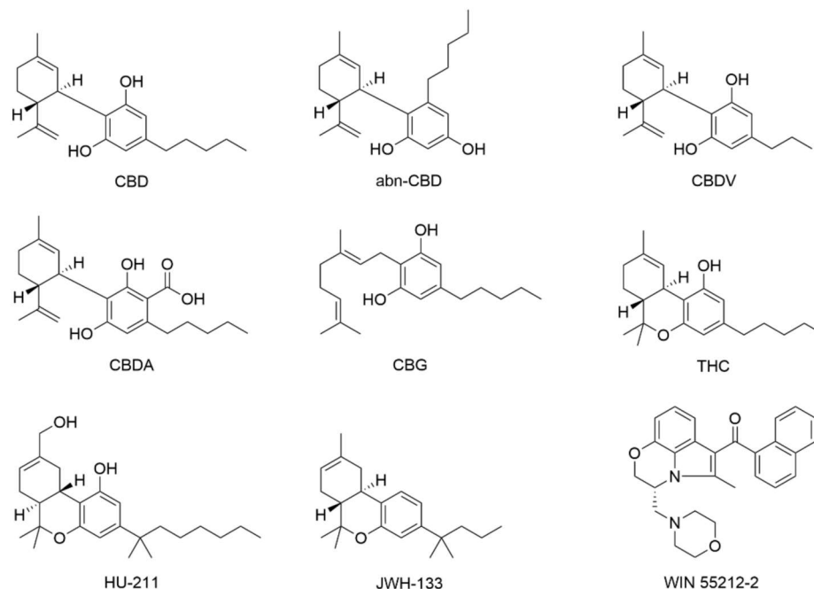
Figure 2. Chemical structures of cannabinoids and their synthetic analogs discussed in this review.
