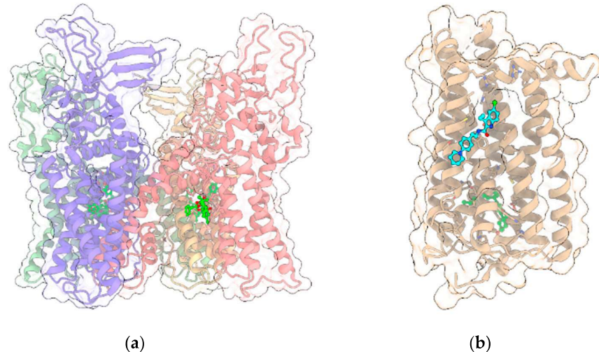
Figure 3. (a) Crystal structure (PDB entry: 5IRX) of the 4:4 complex between rat TRPV1 (light green, red, yellow and violet ribbon and transparent surface for the four protein monomers) and the agonist resiniferatoxin (ball and stick with bright green C atoms); (b) Crystal structure (PDB entry: 6KQI) of the complex of CB1R (tan ribbon and transparent surface) with the negative allosteric modulator ORG27569 (ball and stick with cyan C atoms) and the agonist CP55940 (ball and stick with bright green C atoms). In all panels, other ligands and non-receptor protein sequences are omitted; protein sidechains contacting ligands within 5 Å are shown as sticks; oxygen, nitrogen, sulfur and chlorine atoms in ligands and visible protein sidechains are colored red, blue, yellow and green, respectively.
