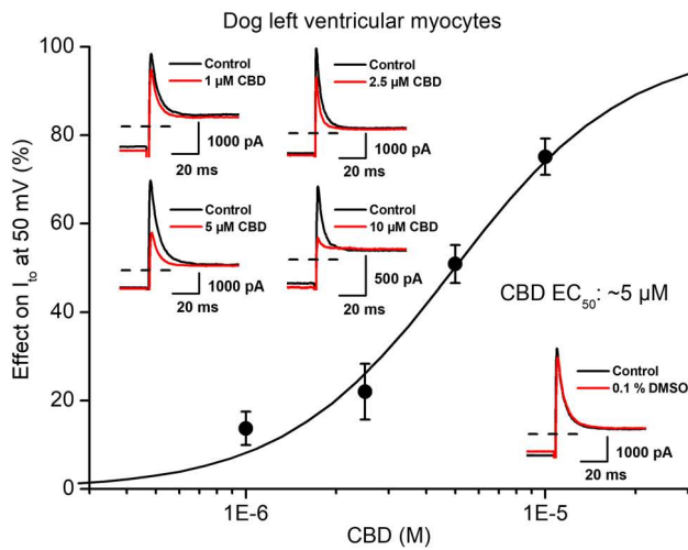
Fig. 6 Effect of CBD on the transient outward potassium current ( I_{to} ) in dog ventricular myocytes. The panel displays CBD concentration–response curve indicating an estimated EC_{50} value of 5 \mu\text{M} for I_{to} blockade. Insets show original I_{to} current traces in control conditions and in the presence of 1 \mu\text{M} , 2.5 \mu\text{M} , 5 \mu\text{M} and 10 \mu\text{M} CBD recorded from dog left ventricular myocytes after a 300 ms long pulse to 50 mV test potential with pulsing cycle length of 3 s. The inset on right-bottom displays original I_{to} current traces in control conditions and in the presence of the solvent (0.1% DMSO). Dashed lines indicate zero current levels. Data are expressed as means \pm SEM
