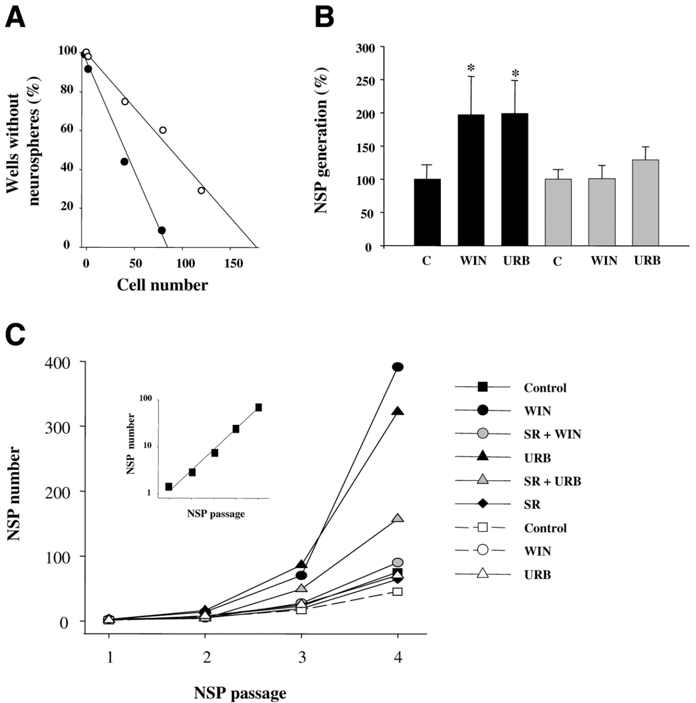
Figure 3. Impaired neurosphere generation in CB 1 knockout mice. A) Limit dilution analysis of neurosphere generation activity in CB 1 -deficient mice (○) and their wild-type littermates (●). B) Effect of WIN-55,212-2 and URB597 on neurosphere-forming cells derived from wild-type (black bars) and CB 1 -knockout mice (gray bars). C) Self renewal of NPs derived from wild-type (solid lines) and CB 1 -knockout mice (dashed lines). Number of neurospheres was quantified after 4 consecutive neurosphere passages in the continuous presence of the indicated stimuli. Inset) Representative logarithmic plot of neurosphere generation. Results correspond to 4 ( A , B ) or 3 ( C ) independent experiments. Significantly different from controls: * P < 0.05.
