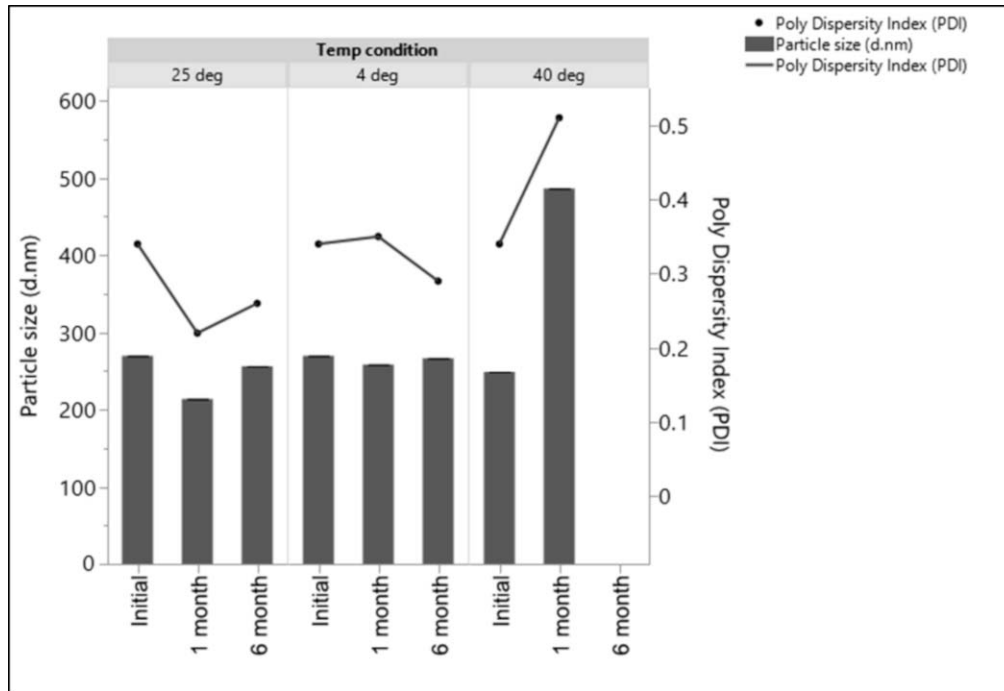
Figure 3. Particle size and polydispersity index of THC-VHS-SLNs stored at conditions of 40°C/60% RH, 25°C/75% RH, and 4°C over a period of 6 months.
